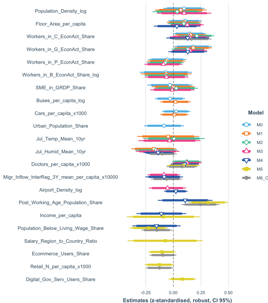
Fig. 2. Comparison of the coefficients of the models M0-M6_C
